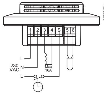
Connections MTC2-1991 (setback)
