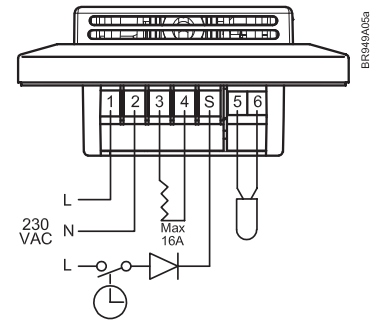
Connections OTD2-1999 (frost protection mode)
